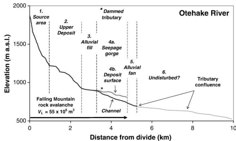
Fig. 9. Long profile of 1929 Falling Mountain rock avalanche (WSA, New Zealand), which catastrophically infilled W Branch Otehake River up to \sim 80 m without major blockage. The river incised a 2-km long gorge into the fragmented and easily erodible debris downstream of several seepage springs. Numbers refer to Fig. 8.
