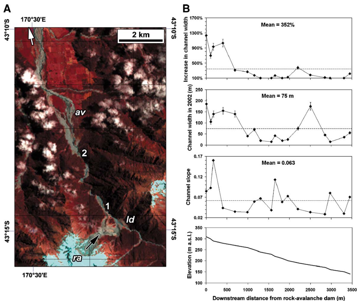
Fig. 10. (A) Landsat ETM+ subsense (path 75, row 90; bands 5, 3, 2 RGB; 31 December 2002) of 1999 Mt. Adams rock avalanche, WSA, New Zealand; ra=rock avalanche (black → indicates failure movement); ld=breached landslide dam; av=landslide-induced fanhead avulsion. (B) Downstream variation of channel geometry in Poerua gorge between “1” and “2” (white → indicates flow). Elevation and gradient data refer to pre-1999 channel. Channel width w and its relative increase were measured from 1984 and 2002 air photographs at \pm 10\% accuracy. Image courtesy of Global Land Cover Facility, University of Maryland.
