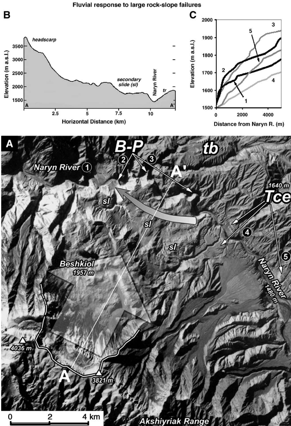
Fig. 2. (A) KFA-1000 satellite subscene (FN 1051/Frame 21626) of the giant ( 10^{10} \text{ m}^3 ) Beshkiol rockslide dam on Naryn River, Kyrgyz Tien Shan, forming a 70-km long lake (inferred from lake terraces, Tce). Curved \rightarrow = inferred former river course. Fluvial response involved cutting of a 10-km long and 300-m deep bypass gorge (B–P) into hard Palaeozoic rocks of a tectonic bench (tb); sl = secondary landslides; 1–5 = tributaries (see C). (B) Long profile of rockslide. (C) Contrast in tributary long profiles showing fluvial hanging valleys because of delayed response to rapid gorge incision (1–3), and more adjusted tributaries (4–5) responding to gradual backwater aggradation.
